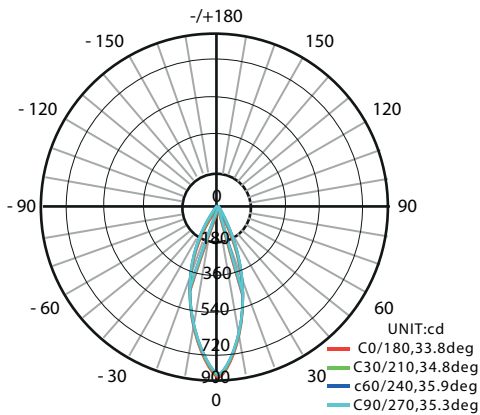
AVERAGE BEAM ANGLE (50%):34.9 DEG GD1090-AM-3K
