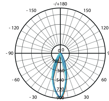
AVERAGE BEAM ANGLE (50%):36.9 DEG GD1070-AM-5K
