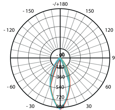
AVERAGE BEAM ANGLE (50%):36.9 DEG GD1070-AM-4K
