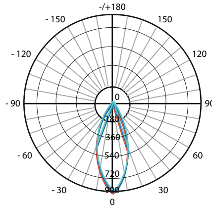
AVERAGE BEAM ANGLE (50%):36.9 DEG GD1090-AM-4K
