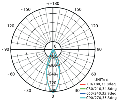
AVERAGE BEAM ANGLE (50%):34.9 DEG GD1070-AM-3K
