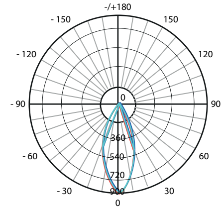
AVERAGE BEAM ANGLE (50%):36.9 DEG GD1090-AM-5K
